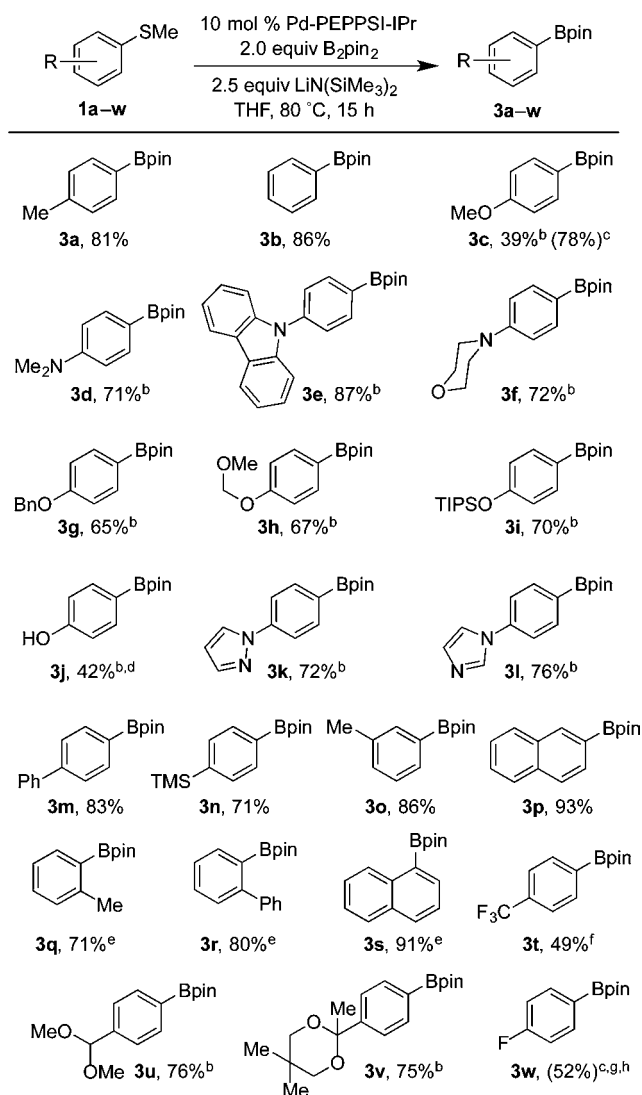
Scheme 1. Palladium-Catalyzed Borylation of Aryl Sulfides with \text{B}_2\text{pin}_2 a
