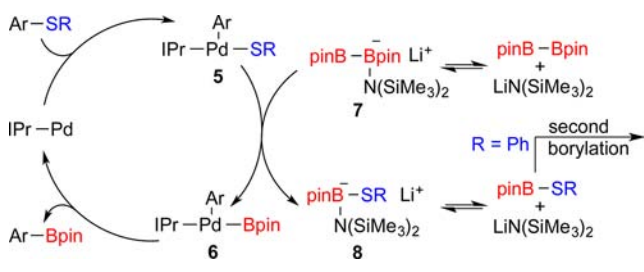
Scheme 4. Plausible Catalytic Cycle
